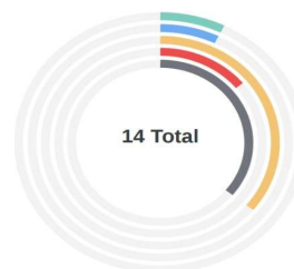
PenTest Findings
